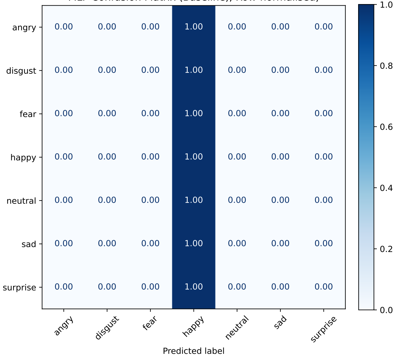
MLP Confusion Matrix (Baseline), Row-normalised)
