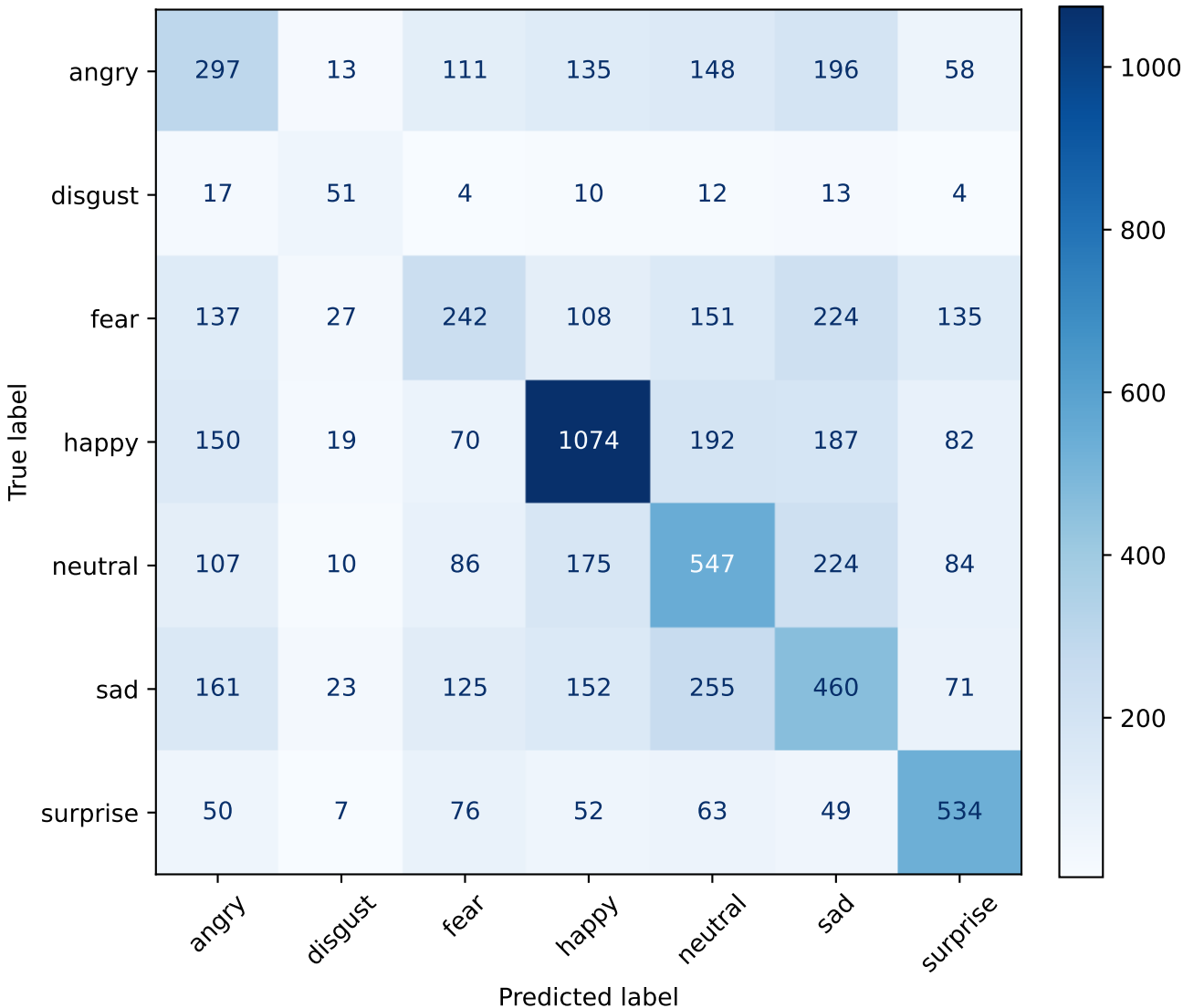
MLP Confusion Matrix (Stabilised, Counts)
