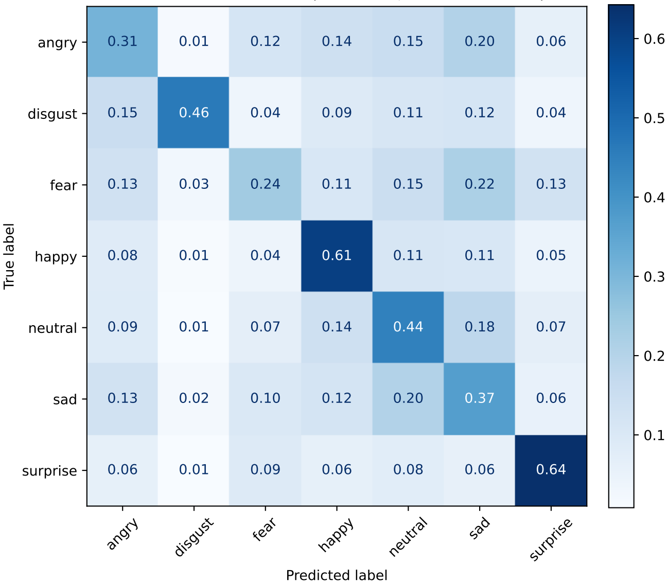
MLP Confusion Matrix (Stabilised, Row-normalised)
