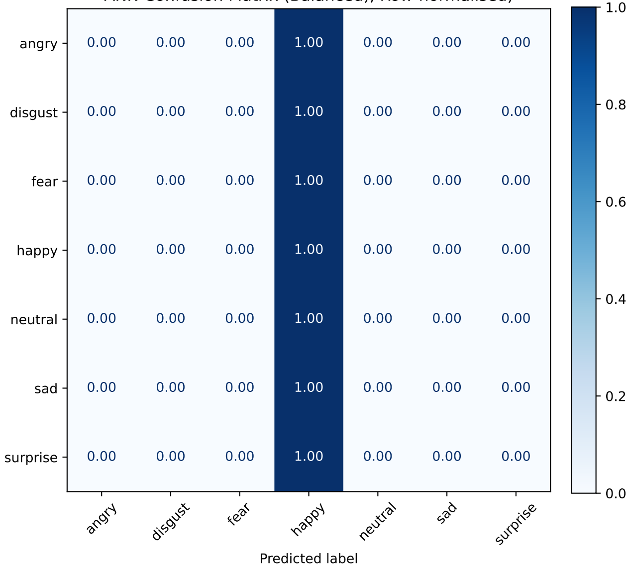
ANN Confusion Matrix (Balanced), Row-normalised)
