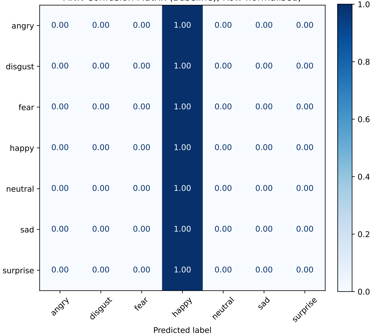
ANN Confusion Matrix (Baseline), Row-normalised)
