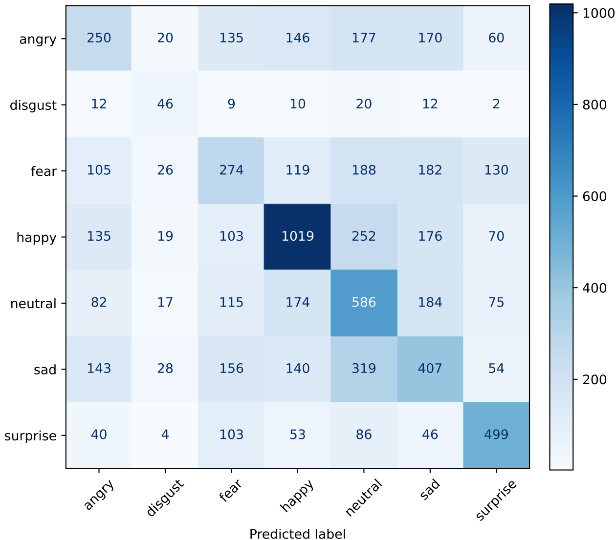
ANN Confusion Matrix (Stabilised, Counts)
