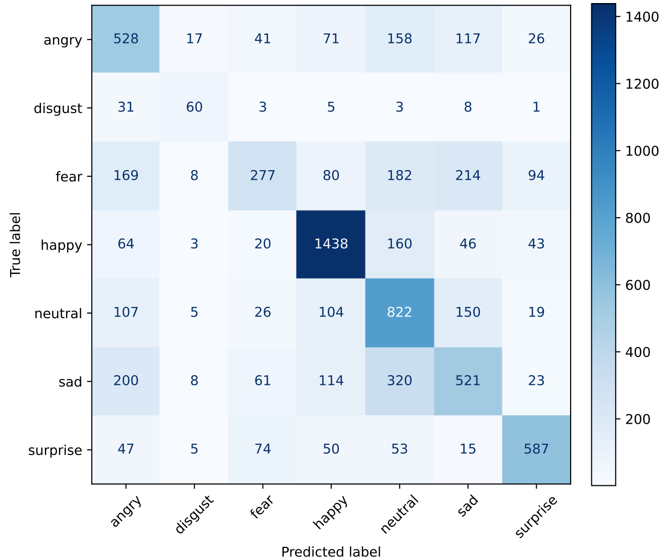
CNN Confusion Matrix (Stabilised, Counts)
