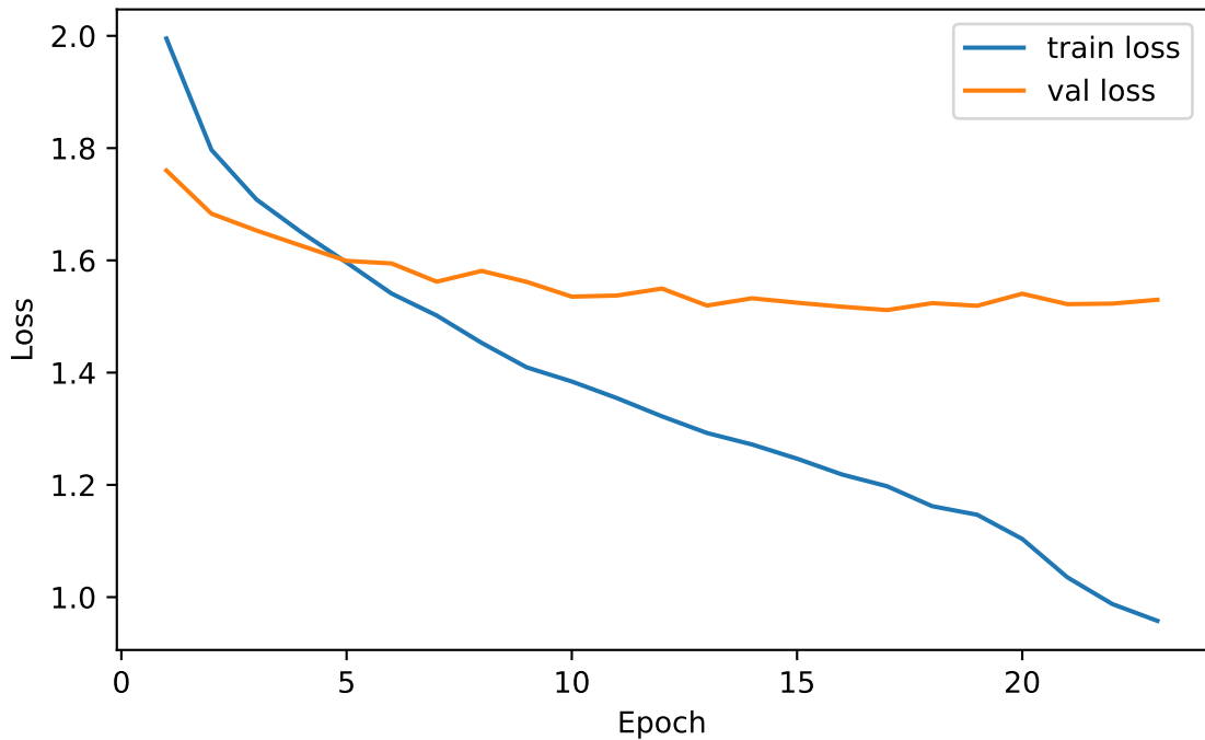
ANN Loss (Stabilised)
