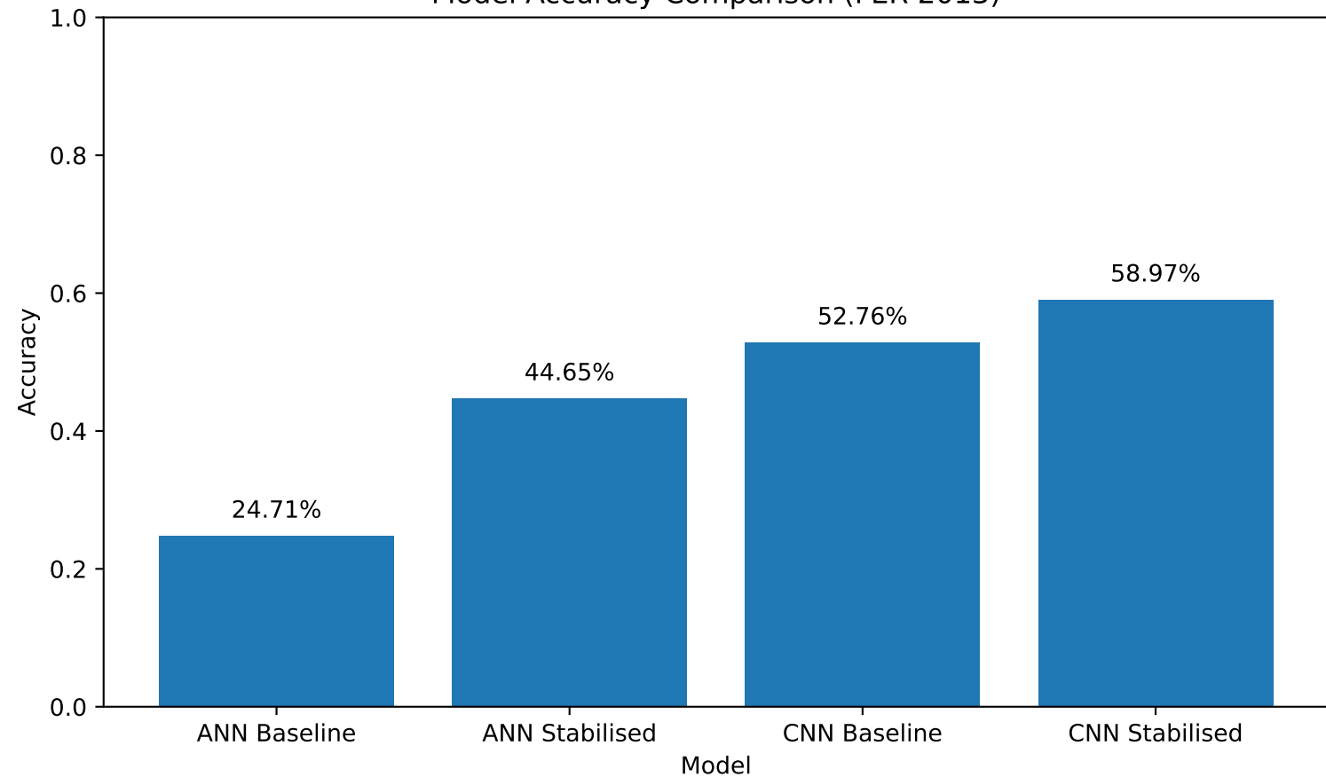
Model Accuracy Comparison (FER-2013)
