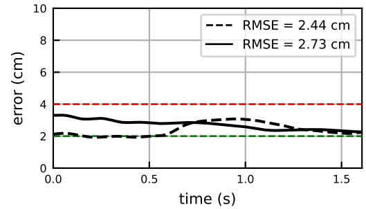
SHO
