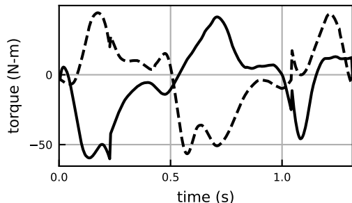
knee_angle_moment
