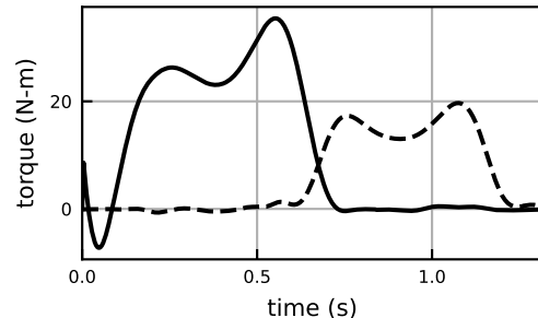
lumbar_bending_moment
