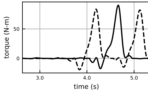
lumbar_extension_moment
