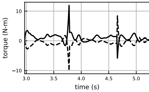
wrist_flex_moment
