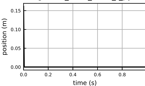
ground_force_calcn_r_py
