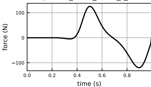
ground_force_calcn_r_px
