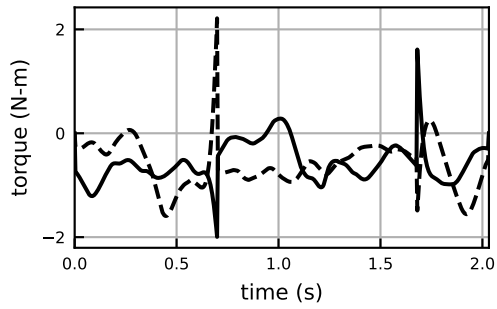
wrist_flex_moment
