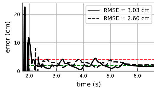
Unnamed: 19
