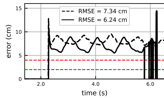
Unnamed: 21
