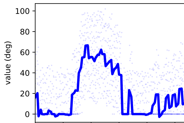
/jointset/walker_knee_r/knee_angle_r/value
