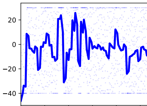
/jointset/ankle_r/ankle_angle_r/value
