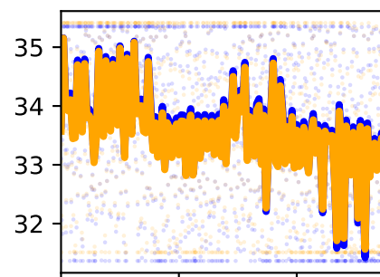
/forceset/soleus_r_length
