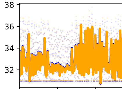
/forceset/addlong_l_length
