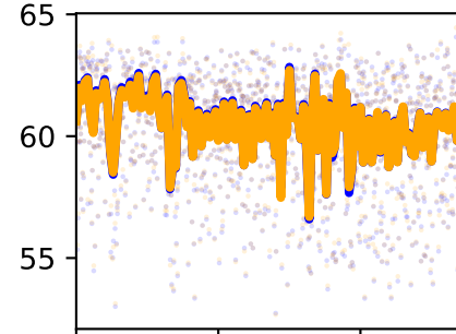
/forceset/tfl_r_length
