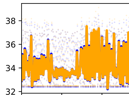
/forceset/addmagDist_l_length
