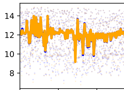
/forceset/addmagProx_l_length
