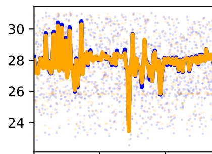
/forceset/addlong_l_length
