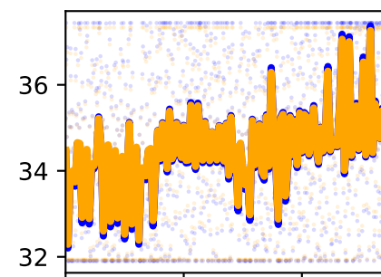
/forceset/tibant_r_length
