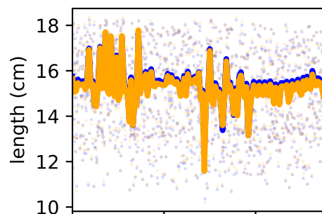
/forceset/addbrev_l_length
