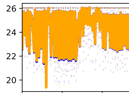
/forceset/bfsh_l_length
