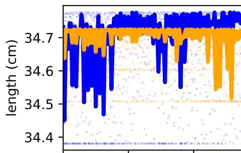
/forceset/addbrev_l_length
