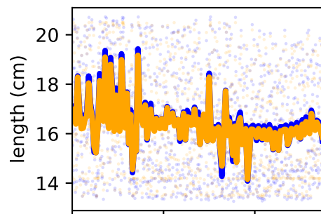
/forceset/addmagMid_l_length
