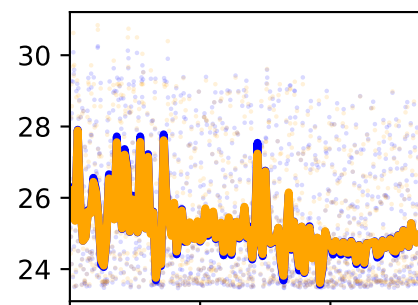
/forceset/addmagDist_l_length
