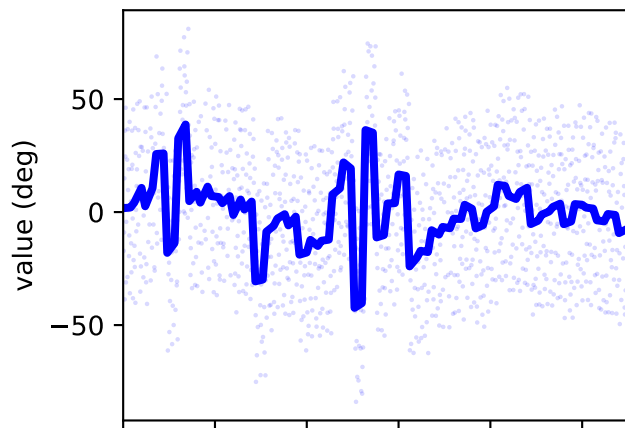
/jointset/acromial_r/arm_rot_r/value
