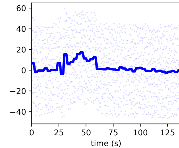
/jointset/acromial_l/arm_rot_l/value
