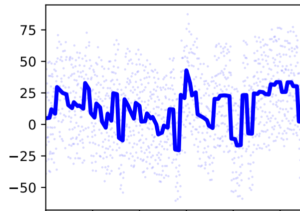
/jointset/back/lumbar_bending/value
