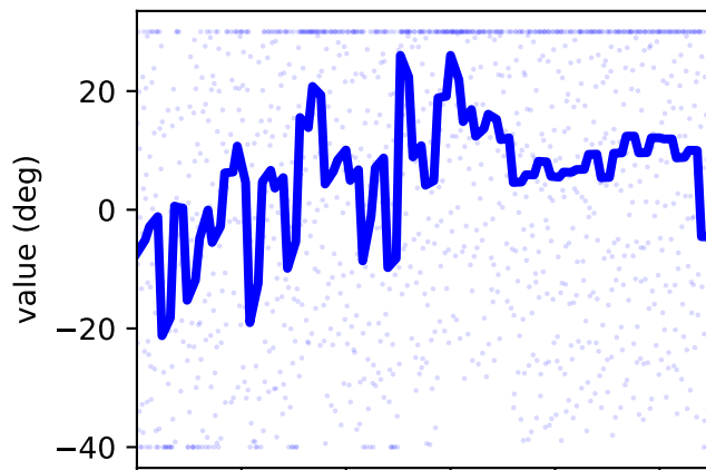
/jointset/ankle_l/ankle_angle_l/value
