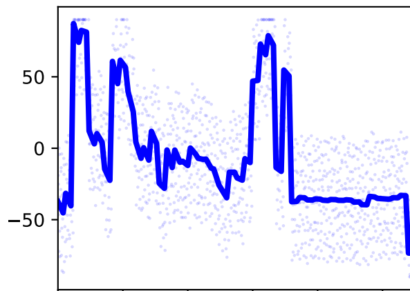
/jointset/back/lumbar_extension/value
