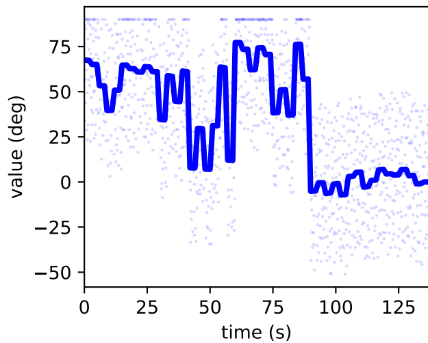
/jointset/acromial_l/arm_flex_l/value
