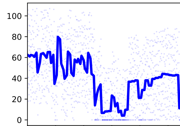
/jointset/walker_knee_l/knee_angle_l/value
