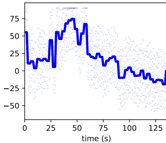
/jointset/acromial_l/arm_add_l/value
