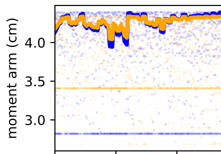
/forceset/gaslat_r_moment_arm_ankle_angle_r
