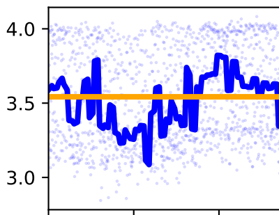
/forceset/fdl_r_moment_arm_ankle_angle_r
