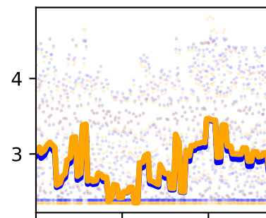
/forceset/fhl_r_moment_arm_ankle_angle_r
