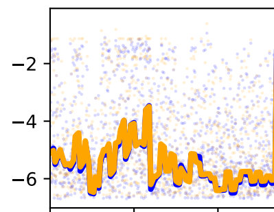
/forceset/bfsh_r_moment_arm_knee_angle_r
