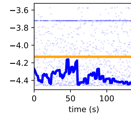
/forceset/gasmed_r_moment_arm_ankle_angle_r
