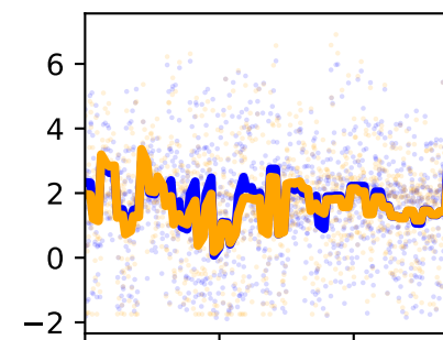
/forceset/edl_r_moment_arm_ankle_angle_r
