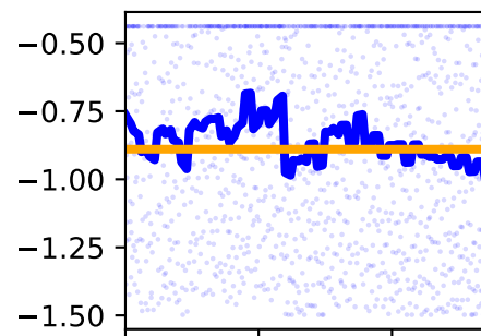
/forceset/gasmed_r_moment_arm_ankle_angle_r
