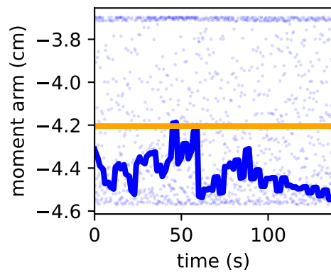
/forceset/gaslat_r_moment_arm_ankle_angle_r
