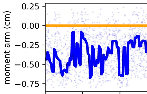
/forceset/ehl_r_moment_arm_ankle_angle_r
