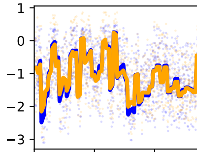
/forceset/bflh_r_moment_arm_knee_angle_r
