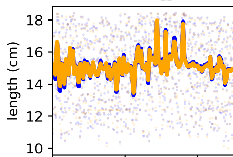
/forceset/addbrev_l_length
