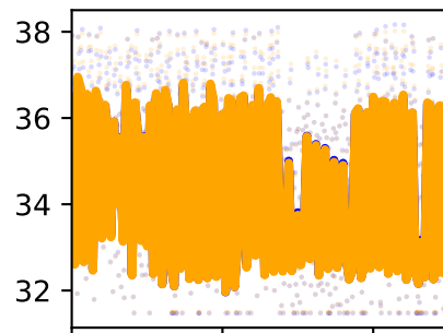
/forceset/vasint_l_length
