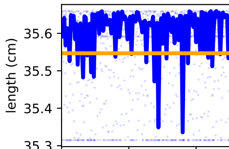
/forceset/tibpost_l_length
