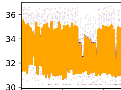
/forceset/vasmed_l_length
