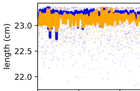
/forceset/semiten_l_length
