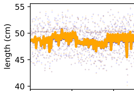
/forceset/tibpost_r_length
