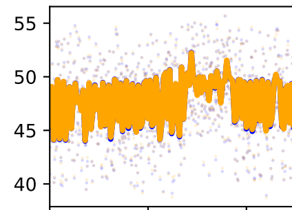
/forceset/grac_l_length
