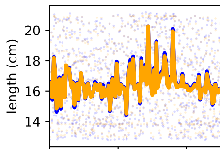
/forceset/addmagMid_l_length
