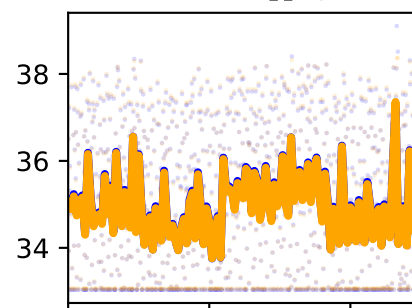
/forceset/addmagDist_l_length
