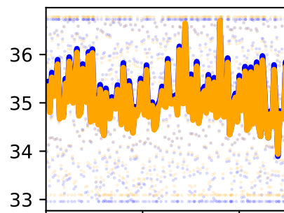
/forceset/soleus_l_length
