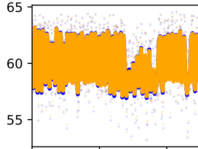
/forceset/soleus_l_length
