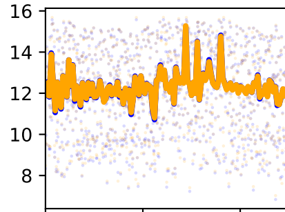
/forceset/addmagProx_l_length
