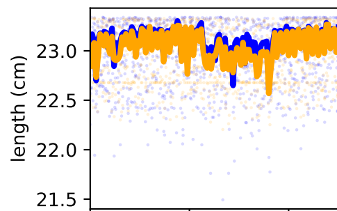
/forceset/psoas_r_length
