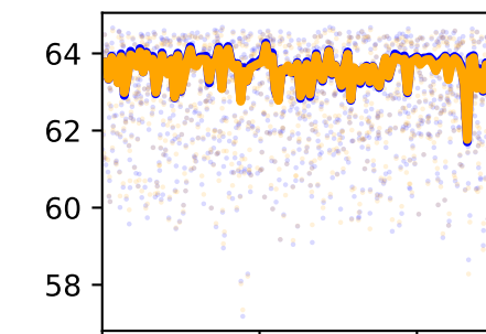
/forceset/sart_r_length
