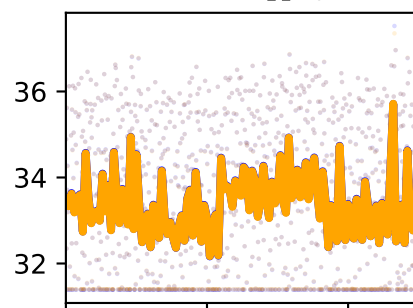
/forceset/addlong_l_length
