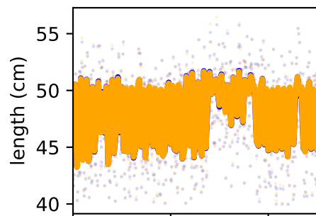
/forceset/semiten_l_length
