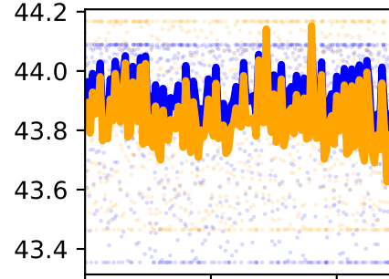
/forceset/sart_l_length
