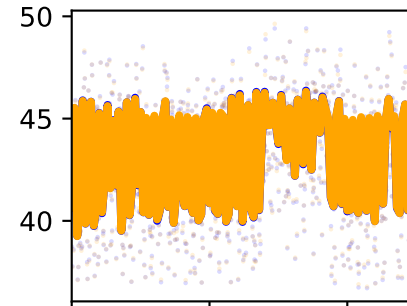
/forceset/tibant_l_length
