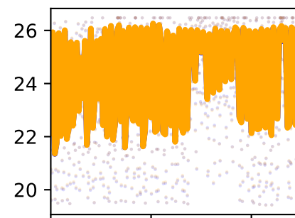
/forceset/bfsh_l_length
