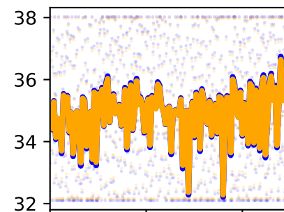
/forceset/tibant_l_length
