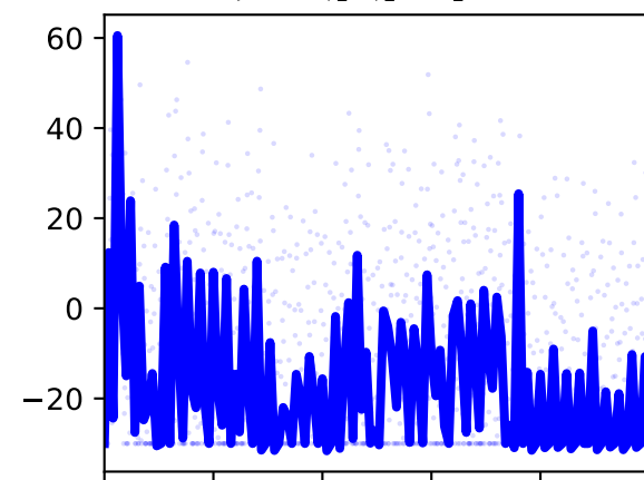
/jointset/walker_knee_l/knee_angle_l/value
