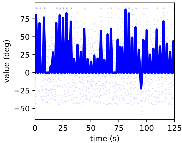
/jointset/acromial_l/arm_flex_l/value
