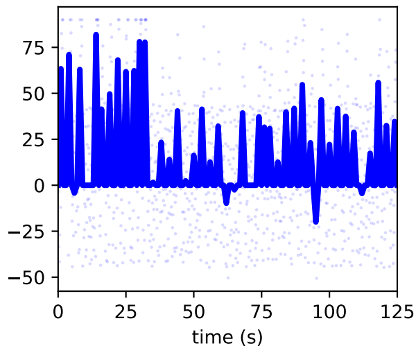
/jointset/acromial_l/arm_add_l/value
