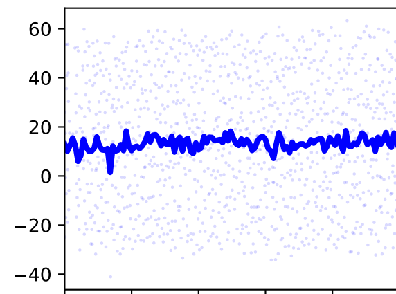
/jointset/ground_pelvis/pelvis_tz/value
