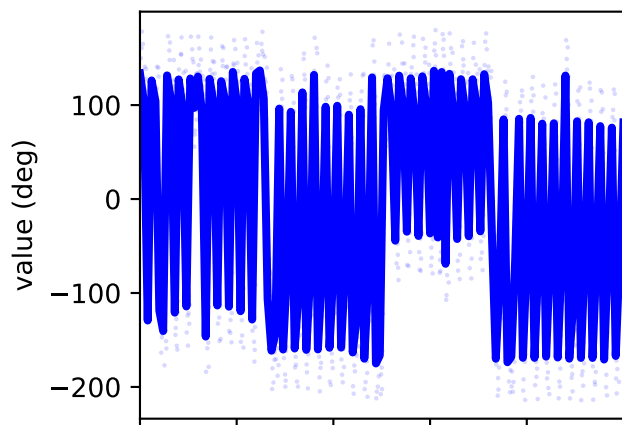
/jointset/ground_pelvis/pelvis_tx/value
