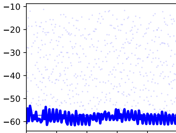
/jointset/ground_pelvis/pelvis_ty/value
