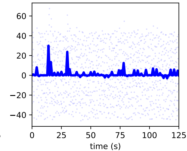
/jointset/acromial_l/arm_rot_l/value
