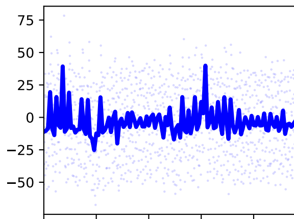
/jointset/ground_pelvis/pelvis_ty/value
