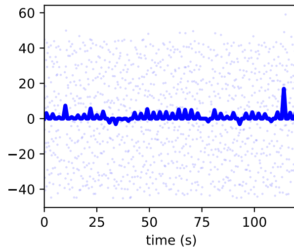
/jointset/acromial_l/arm_rot_l/value
