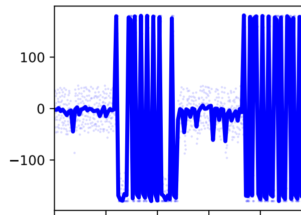
/jointset/ground_pelvis/pelvis_tz/value
