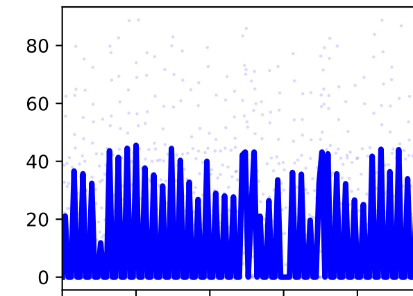
/jointset/acromial_l/arm_rot_l/value
