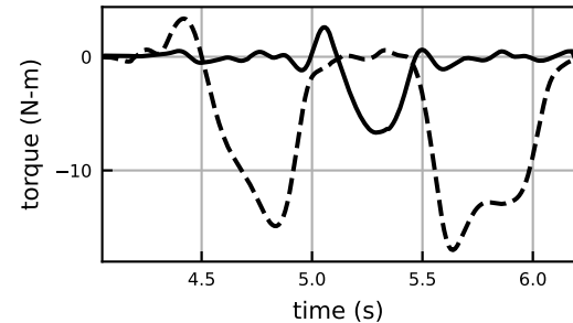
lumbar_bending_moment
