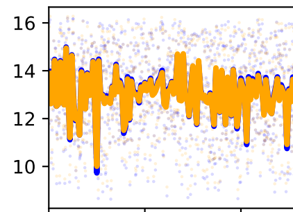
/forceset/semimem_l_length
