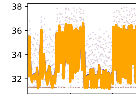
/forceset/vasint_l_length
