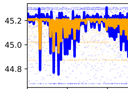
/forceset/fhl_l_length
