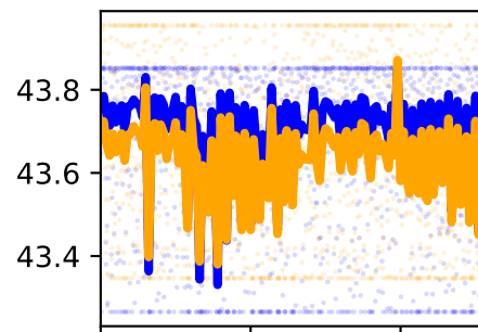
/forceset/sart_l_length
