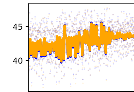
/forceset/semimem_r_length
