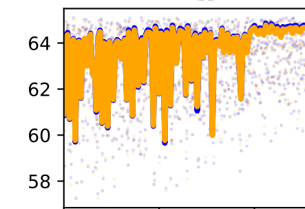
/forceset/sart_r_length
