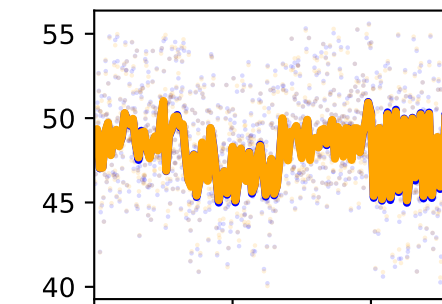
/forceset/grac_l_length
