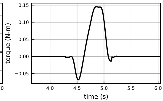
ground_force_calcn_r_mz
