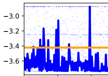
/forceset/gasmed_l_moment_arm_ankle_angle_l
