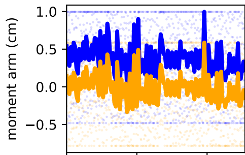
/forceset/fdl_l_moment_arm_ankle_angle_l
