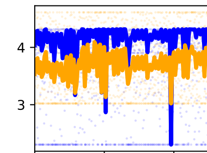
/forceset/edl_l_moment_arm_ankle_angle_l
