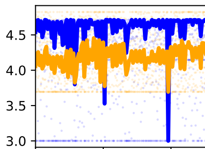
/forceset/ehl_l_moment_arm_ankle_angle_l
