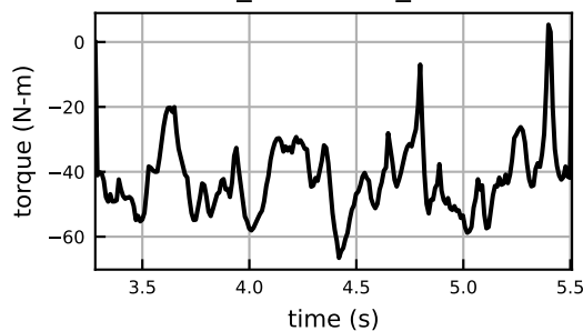
lumbar_extension_moment
