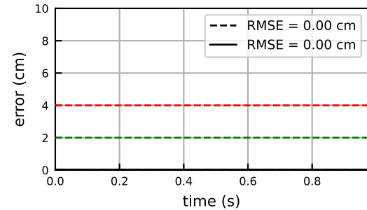
ElbowMoment
