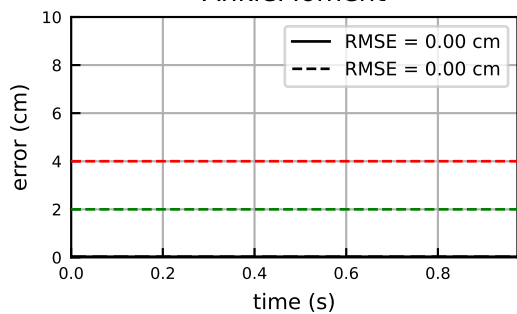
AnkleMoment
