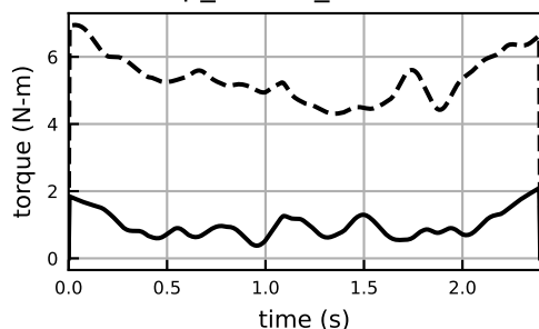
knee_angle_moment
