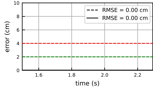
KneeForce
