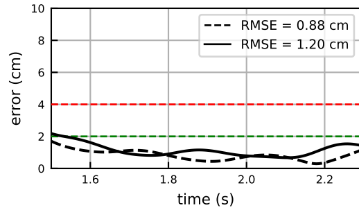
ShoulderMoment
