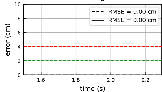
NeckAngles
