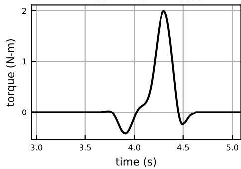
ground_force_calcn_r_my
