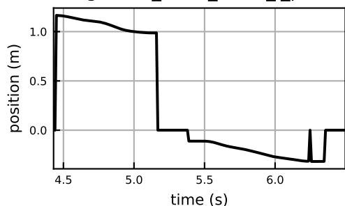
ground_force_calcn_l_mx
