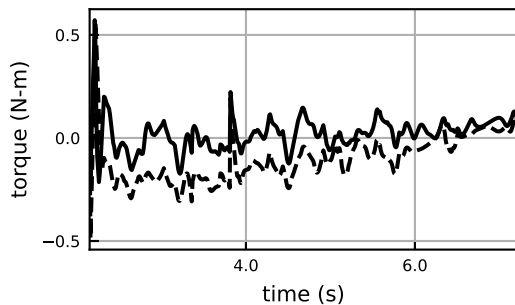
wrist_flex_moment
