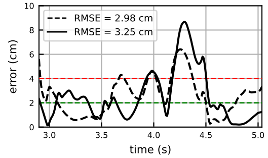
THI
