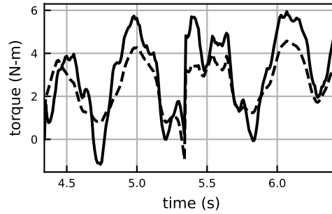
elbow_flex_moment
