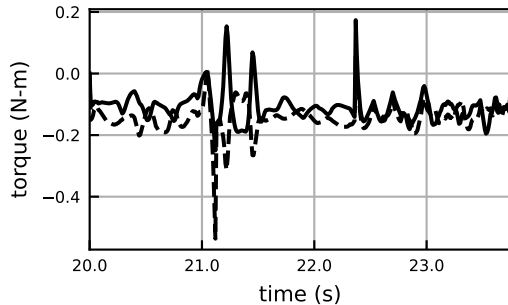
wrist_flex_moment
