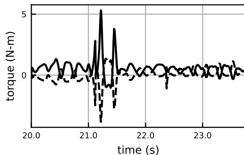
wrist_flex_moment
