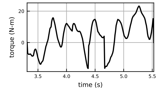
lumbar_bending_moment
