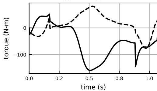
knee_angle_moment
