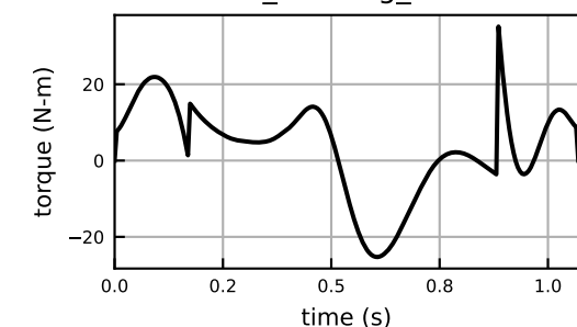
lumbar_bending_moment
