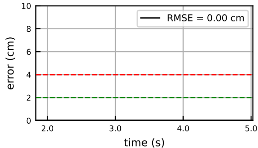
Unnamed: 18
