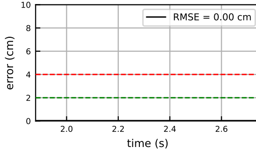
Unnamed: 17
