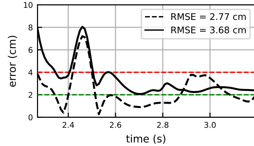
Unnamed: 22
