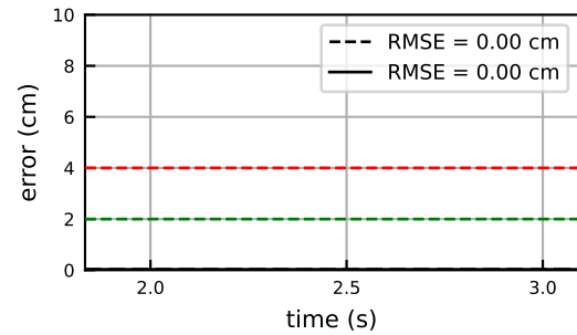
NeckAngles
