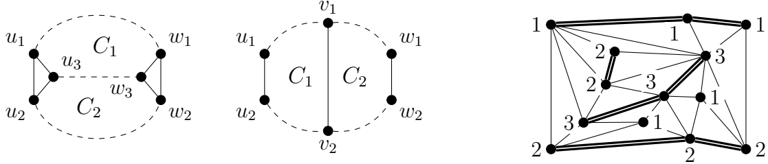
Figure 1: The proof of Lemma 3.1 (left), a graph colored by Poh's algorithm (right).
