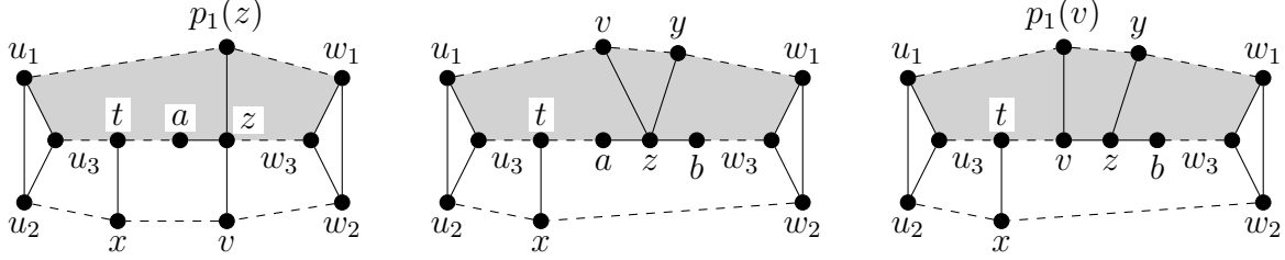
Figure 5: A sketch of Algorithm 3.3 Case 2.2.1 (left), Case 2.2.2 when v \in P_1 (middle), and when v = a (right); in each sketch, the highlighted region represents G_1 .
