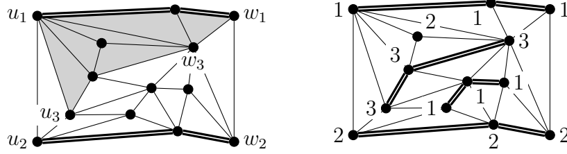
Figure 4: A Poh example highlighting the subgraph G_1 induced by N(P_1) - V(P_2) (left), and the path 3-coloring output from Poh’s algorithm when choosing P_3 = C_1 - P_1 (right).
