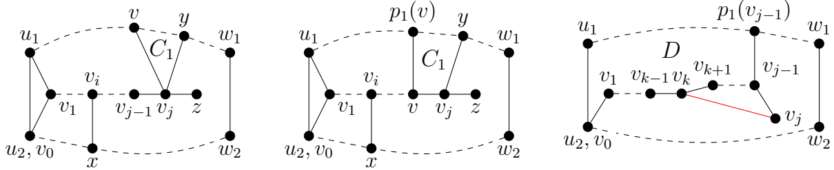
Figure 5: Algorithm 3.3, Case 2.2.2 when v \in P_1 (left) and when v = v_{j-1} (middle). Also, a sketch of why P_3 is an induced path (right).
