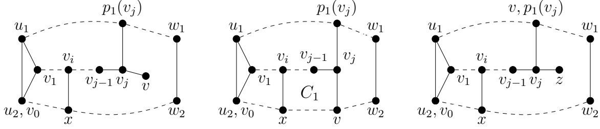
Figure 4: Algorithm 3.3, Case 2.1.1 (left), Case 2.1.2 (middle), and Case 2.1.3 (right).
