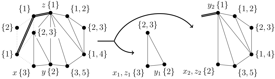
Figure 7: Coloring and removing a path P as in the proof of Lemma 4.1 (Algorithm 4.2).
