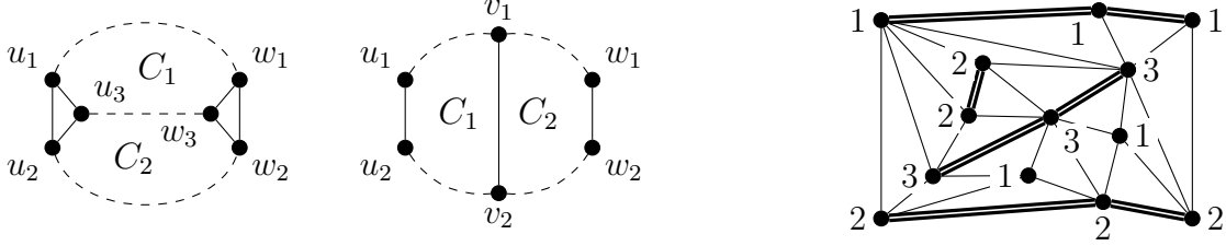
Figure 1: The cases of Lemma 3.1 (left), a graph colored by Poh's algorithm (right).
