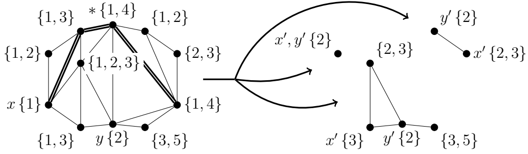
Figure 6: Coloring and removing a path P as in Hartman's proof [7, Lemma 4.2].
