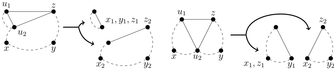
Figure 7: The proof of Lemma 5.1, Case 3.2.1 (left) and Case 3.2.2 (right).
