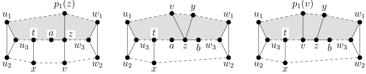
Figure 5: A sketch of Algorithm 3.3 Case 2.2.1 (left), Case 2.2.2 when v \in P_1 (middle), and when v = a (right); the highlighted region represents G_1 .
