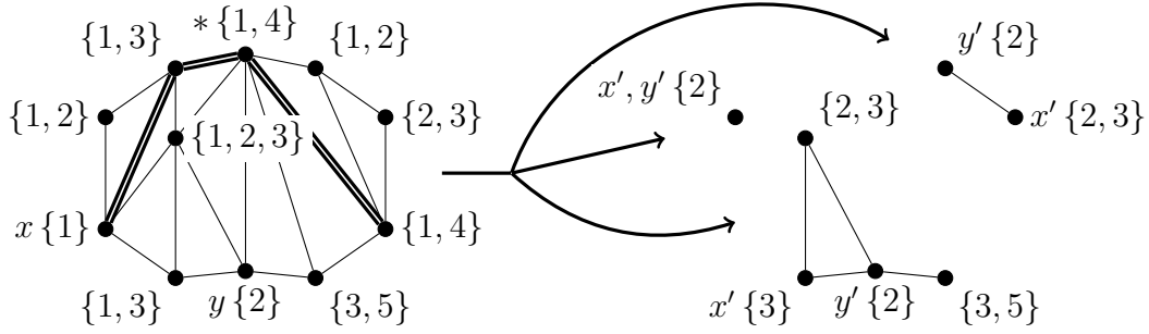
Figure 6: Coloring and removing a path P in the Hartman-Škrekovski algorithm.
