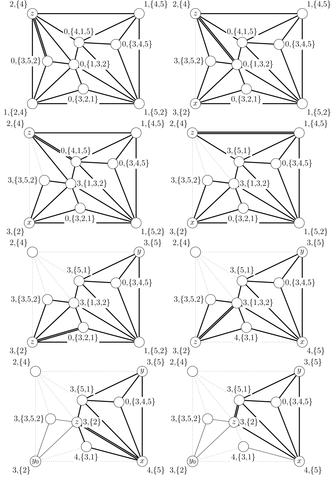
Figure 10: An example of Algorithm 4.2. Each vertex v \in G is labeled with S(v), L(v) .
