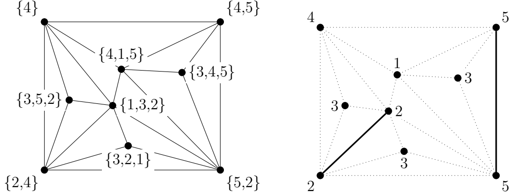
Figure 12: The initial list assignment L (left) and the induced paths of the resulting path L -coloring (right) from the Algorithm 4.2 example shown in Figure 10 and Figure 11.
