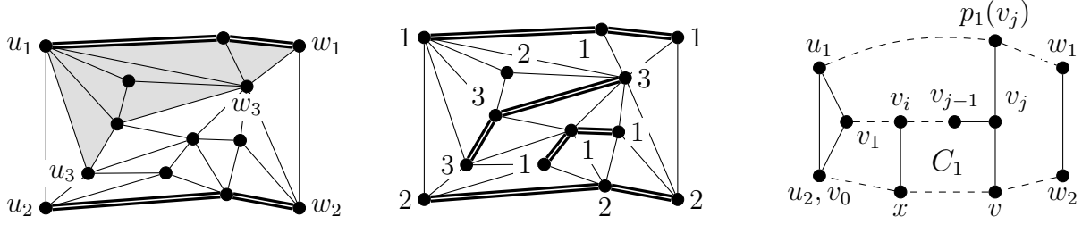
Figure 4: Algorithm 3.3, the subgraph induced by V(P_1) \cup N(P_1) - V(P_2) (left), a path 3-coloring produced by the algorithm (middle), and a sketch of Case 2.1.2 (right).
