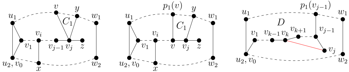
Figure 5: Algorithm 3.3, a sketch of Case 2.2.2 when v \in P_1 (left) and when v = v_{j-1} (middle). Also, a sketch of why P_3 is an induced path (right).
